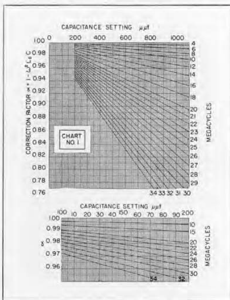
FIGURE 2. Chart No. 1 for determining the quantity \alpha . To facilitate reading the chart at low values of capacitance, the portion below 200 \mu\text{uf} is expanded and plotted below the main chart.
